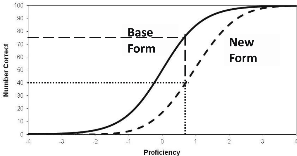
Figure 9.2 Base and new form TCCs.
