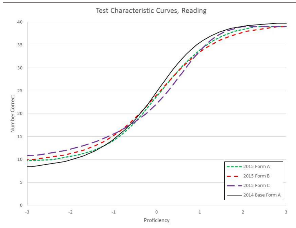
Figure 9.3 Test characteristic curves for Reading.
