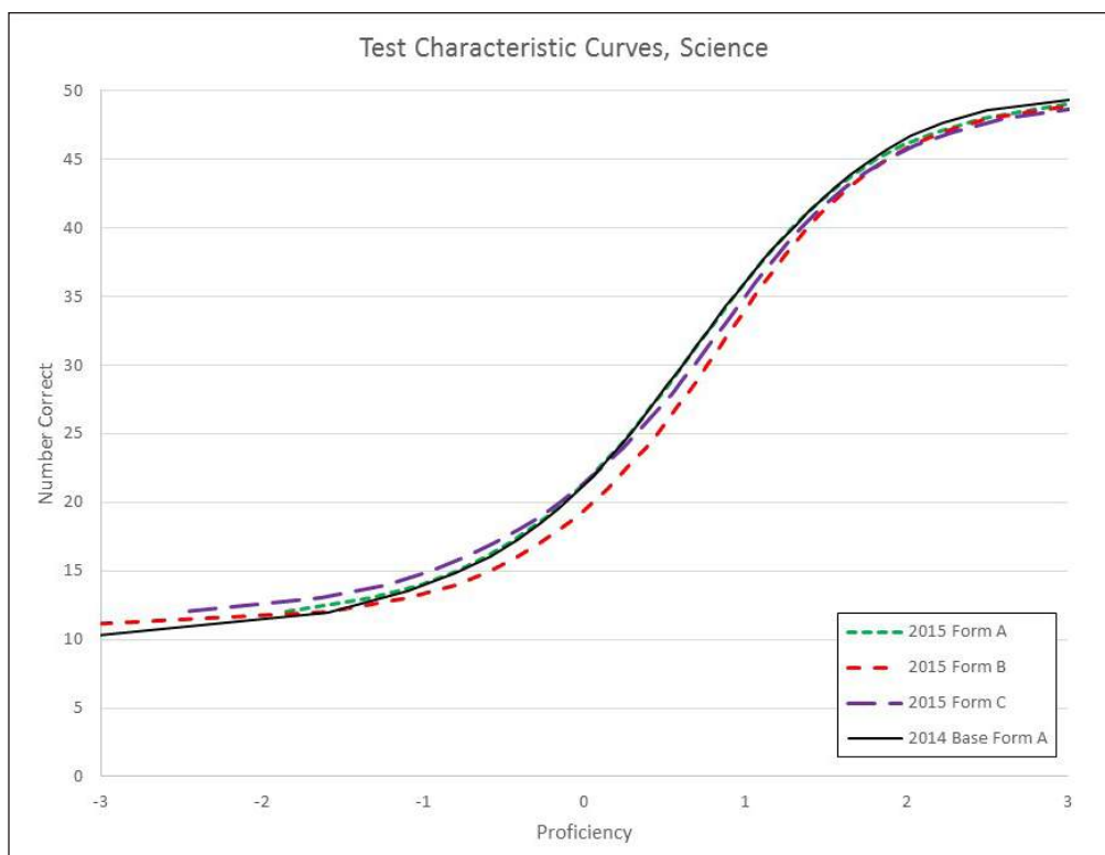
Figure 9.6 Test characteristic curves for Science.
